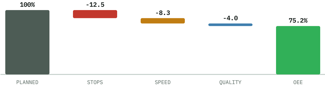
ONE EXAMPLE SHIFT · 480 PLANNED MINUTES · POINTS OF PLANNED TIME
